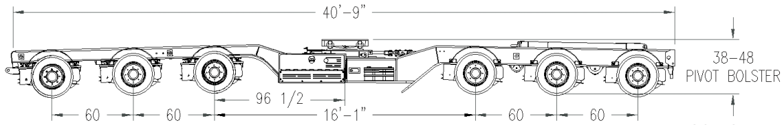
XL 120 DOLLY CAPACITY: 120,000 LB OAL: 40' 9" | OAW: 102"
